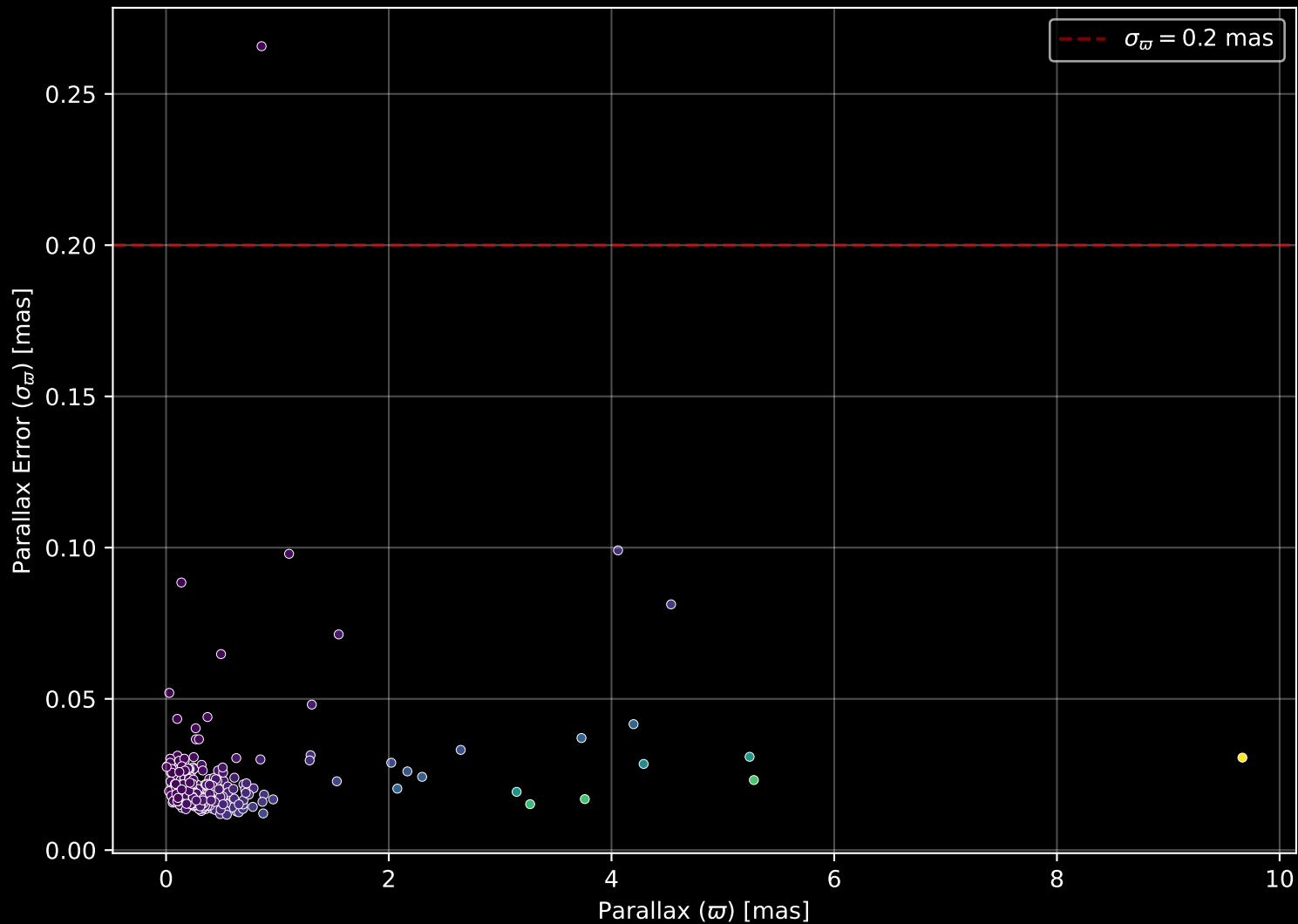
APOGEE DR17 Field: [350-12] Parallax Quality (n= 294)
