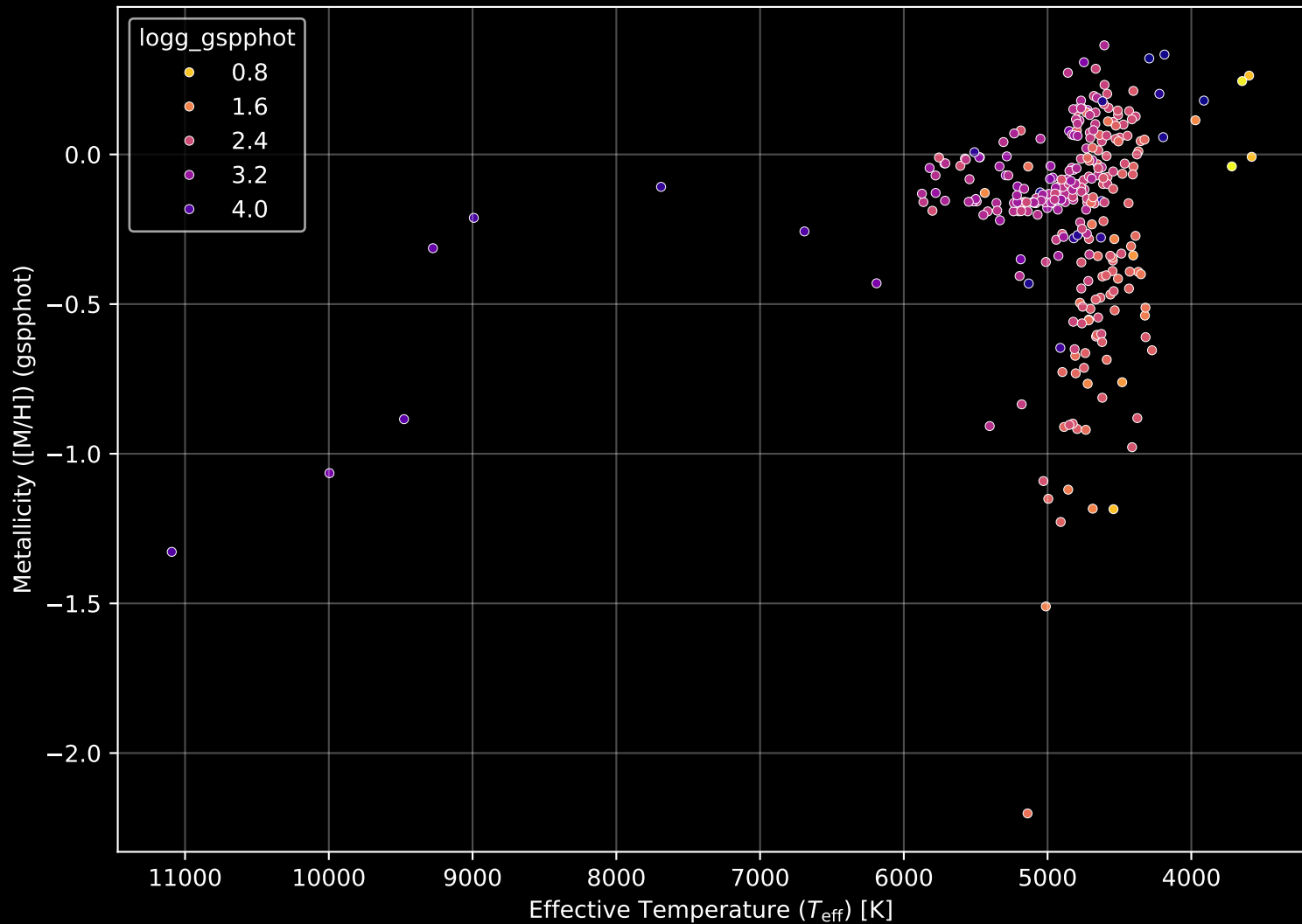
APOGEE DR17 Field: [350-12] Stellar Population Parameters (n= 294)
