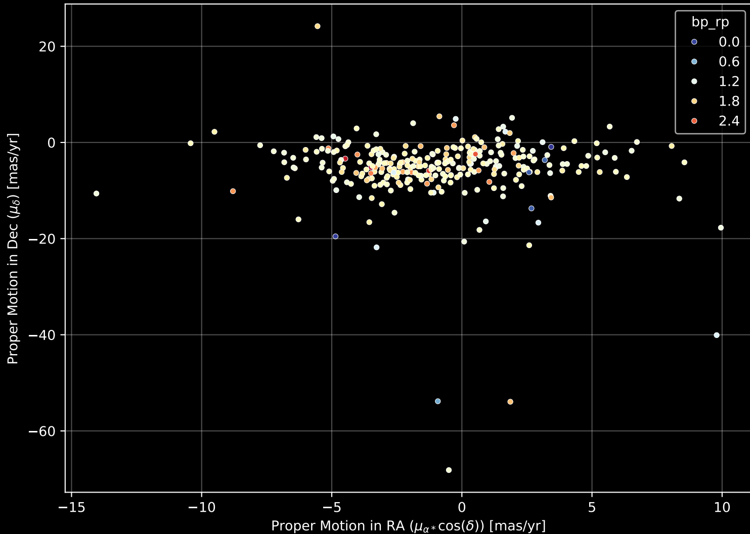
APOGEE DR17 Field: [350-12] Proper Motion Diagram (n= 294)
