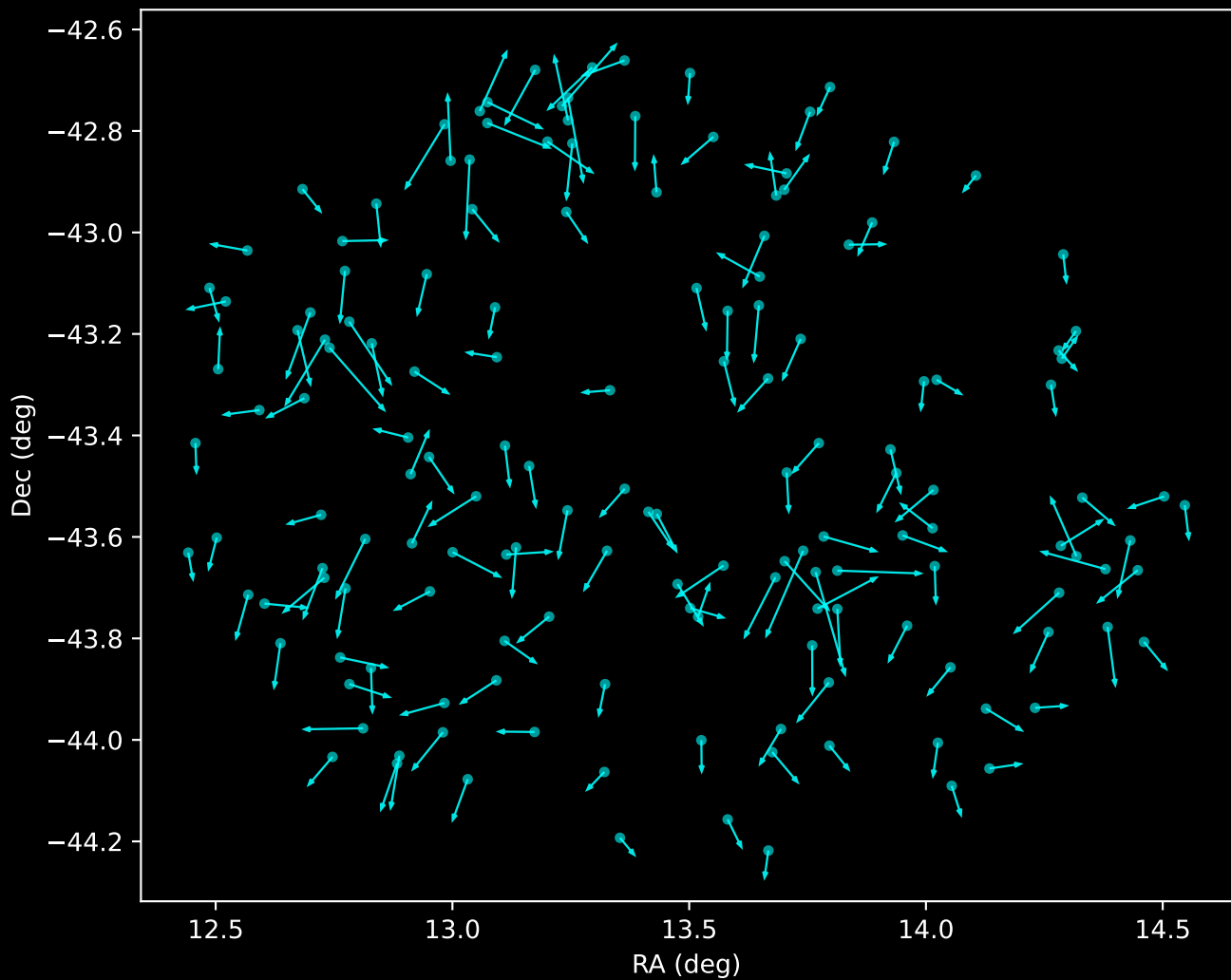
APOGEE DR17 Noise Stream Proper Motion Vectors (n=156)
