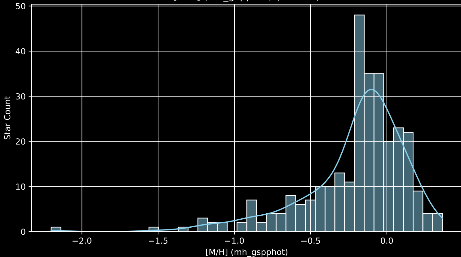
APOGEE DR17 Field: [350-12 [M/H] (mh_gspphot) (n= 294)
