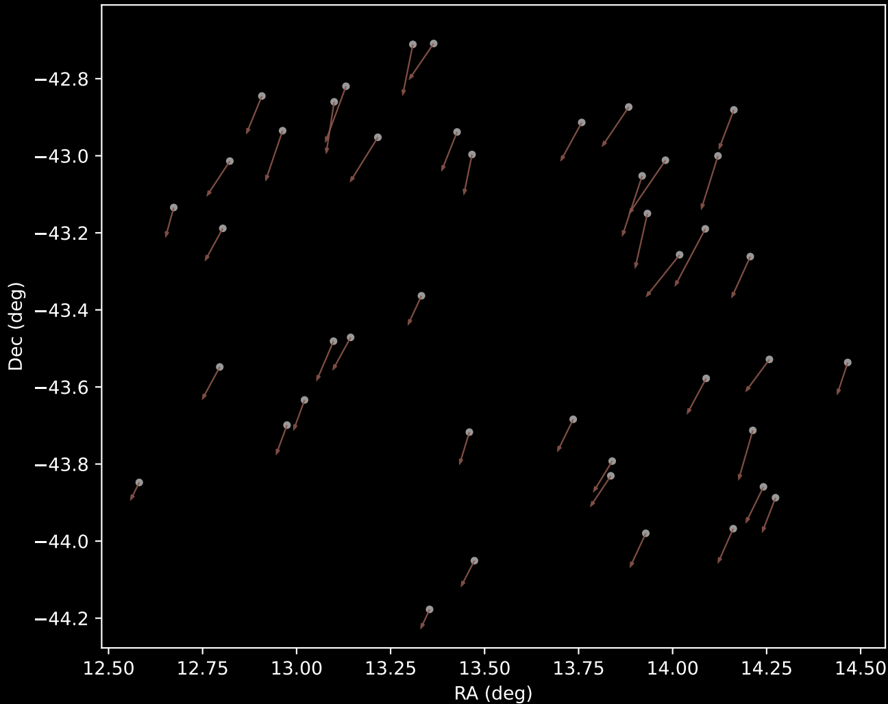
APOGEE DR17 Cluster 10 Proper Motion Vectors (n=43)
