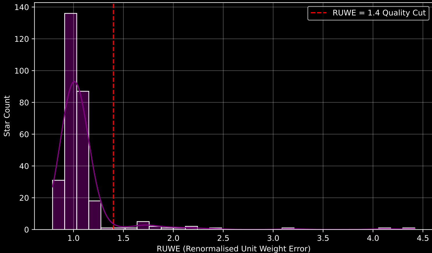
GAPOGEE DR17 Field [350-12] RUWE Distribution (n= 290)
