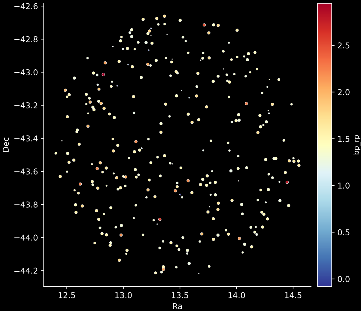
APOGEE DR17 Field: [350-12] Stars: 294
